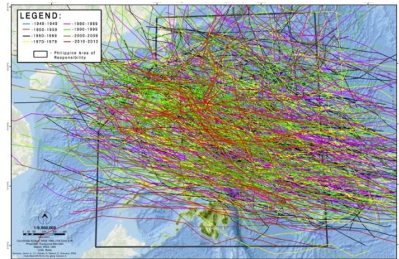
Figure 2. Tracks of tropical cyclones that entered PAR from 1951-2013 (Project NOAH)
