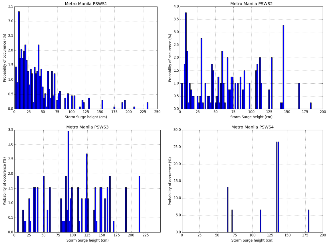
Figure 6. Frequency distribution table for PSWS #1, 2, 3, and 4 of Metro Manila
