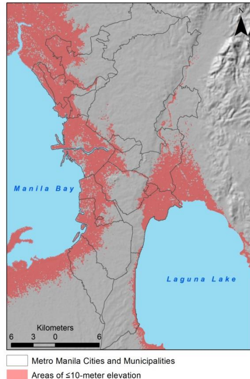
Figure 3. 10-meter Low Elevation Coastal Zone in Metro Manila
