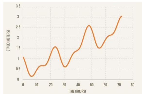
Figure 5. Example storm tide of Metro Manila
