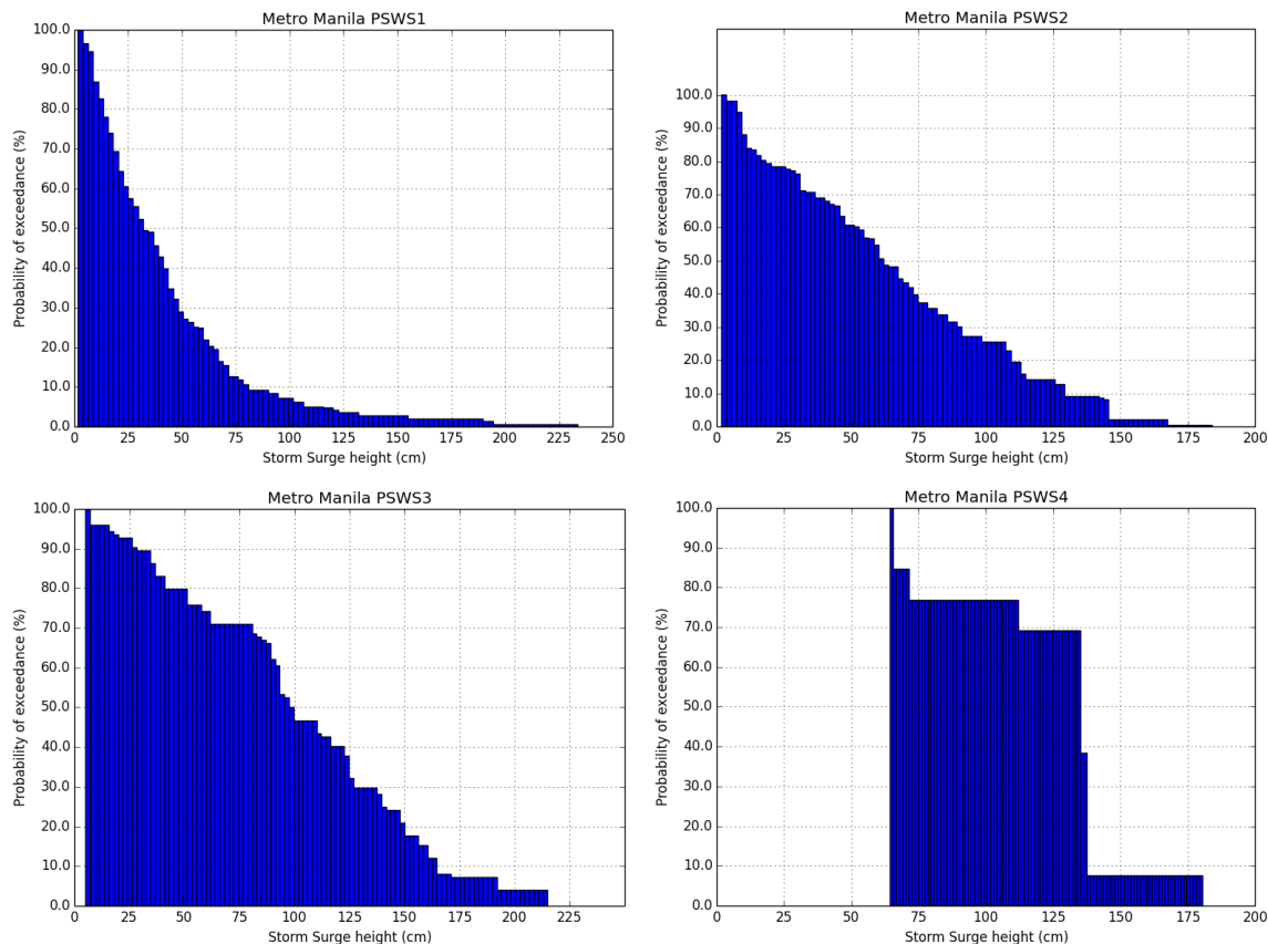
Figure 7. Exceedance probability curve for PSWS #1, 2, 3, and 4 of Metro Manila
