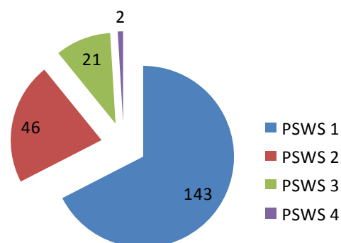
Figure 4. PSWS Frequency Distribution for Metro Manila
